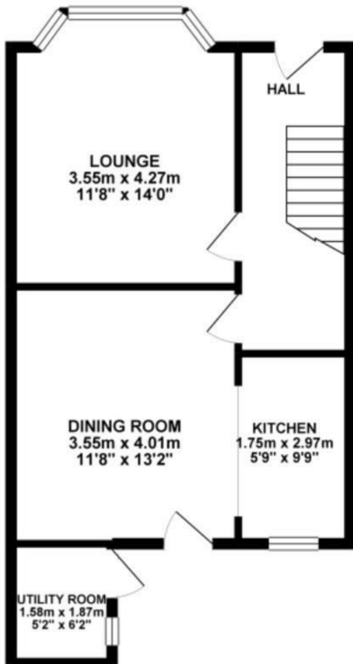
GROUND FLOOR 45.30 sq. m. ( 487.55 sq. ft. )
